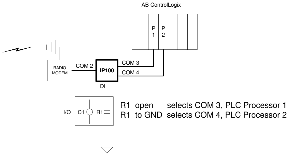
Figure 1: RS-232 Switching between redundant PLC Processors
