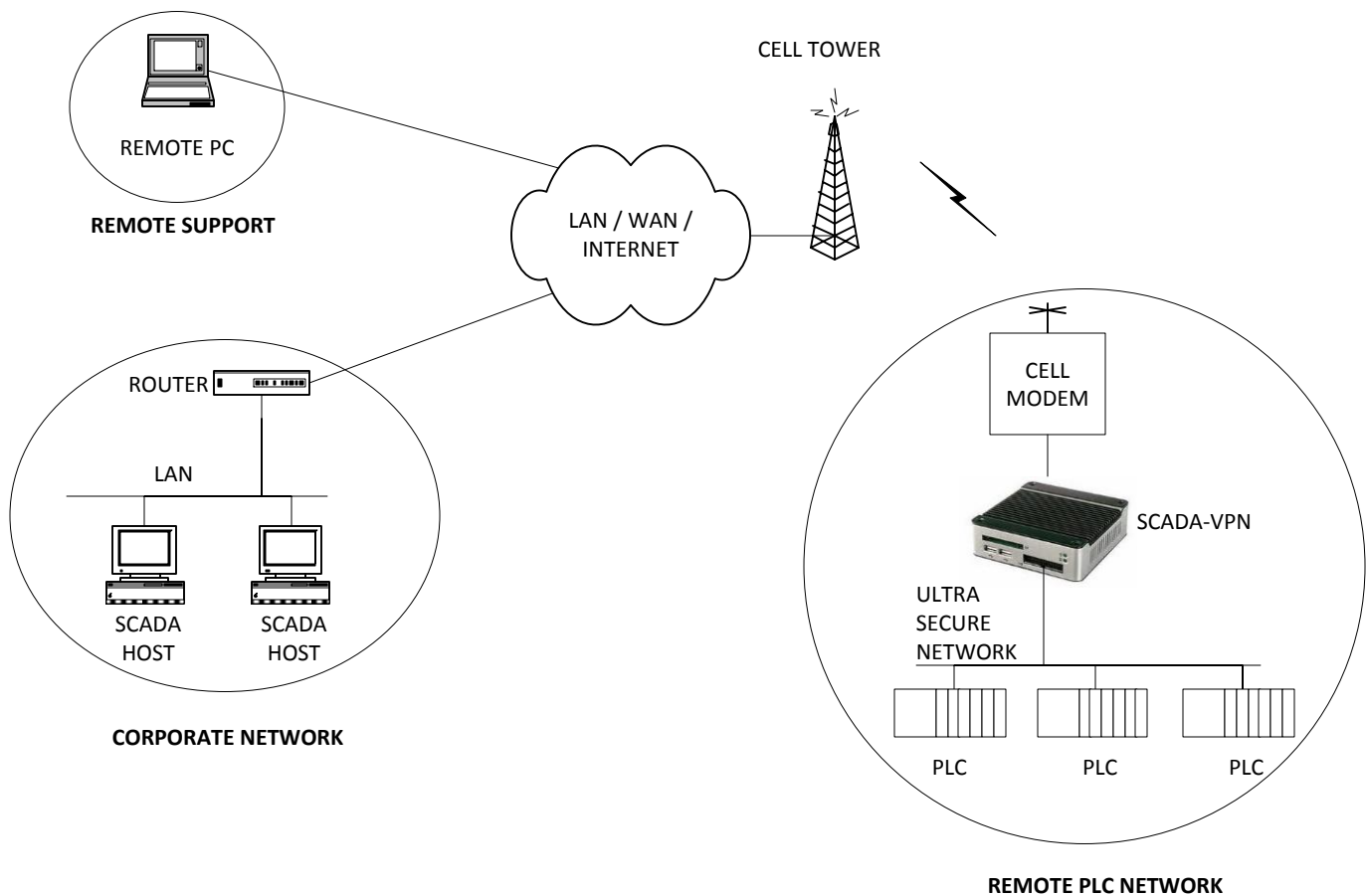
Figure 1: SCADA-VPN for Secure Remote PLC Network Access
