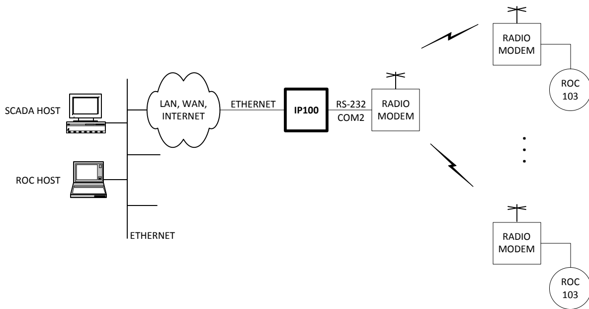
Simultaneous SCADA Polling and ROC Diagnostics using IP100
